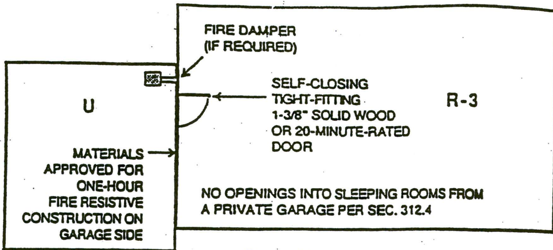
Floor Plan
